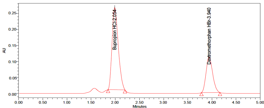
Fig. 4. Chromatogram of standard
