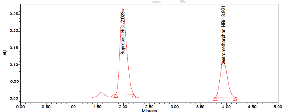
Fig. 6. Chromatogram of sample
