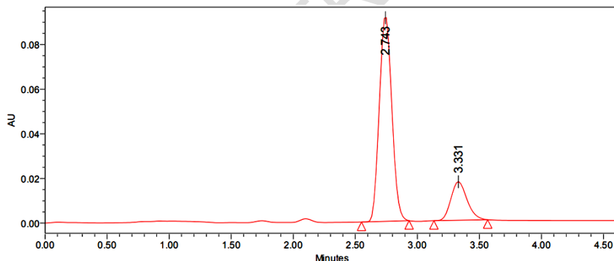
Fig. 2. Chromatogram of trial-1
