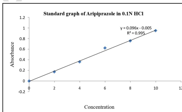
Figure1. StandardgraphofAripiprazolein0.1NHCl
