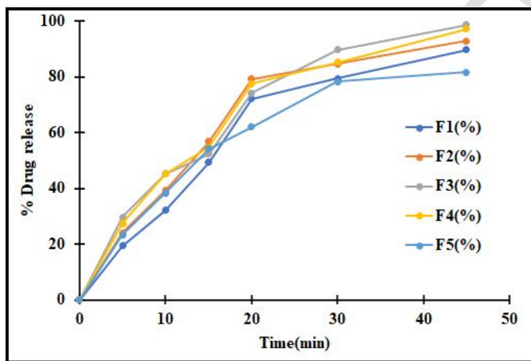
Figure8.DissolutionprofileofAripiprazoleoraldisintegratingtabletsfrom F1 toF5
