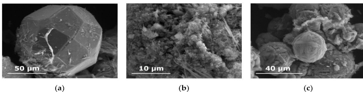
Fig. 7. Microstructures of zeolites obtained in hydrothermal conditions at elevated pressure:
