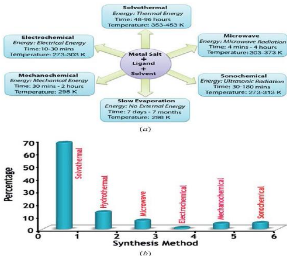
Fig. 9. Synthetic conditions commonly used for MOF preparation (b) summary of the percentage of MOFs synthesized using the various techniques [86]
