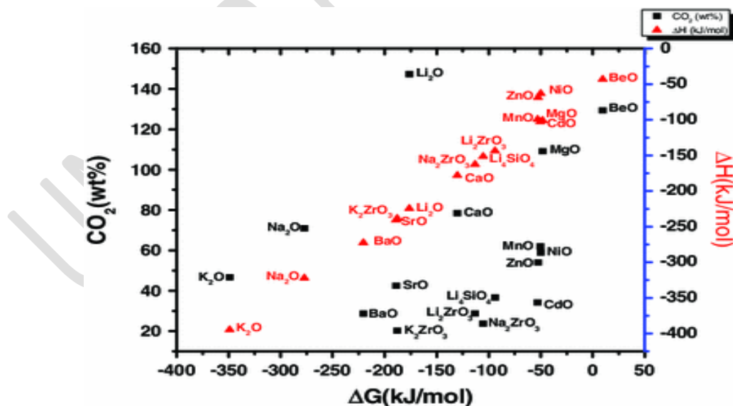
Fig 4: Thermodynamic properties and CO 2 wt% absorbed by different metal oxides at 300K [36]
