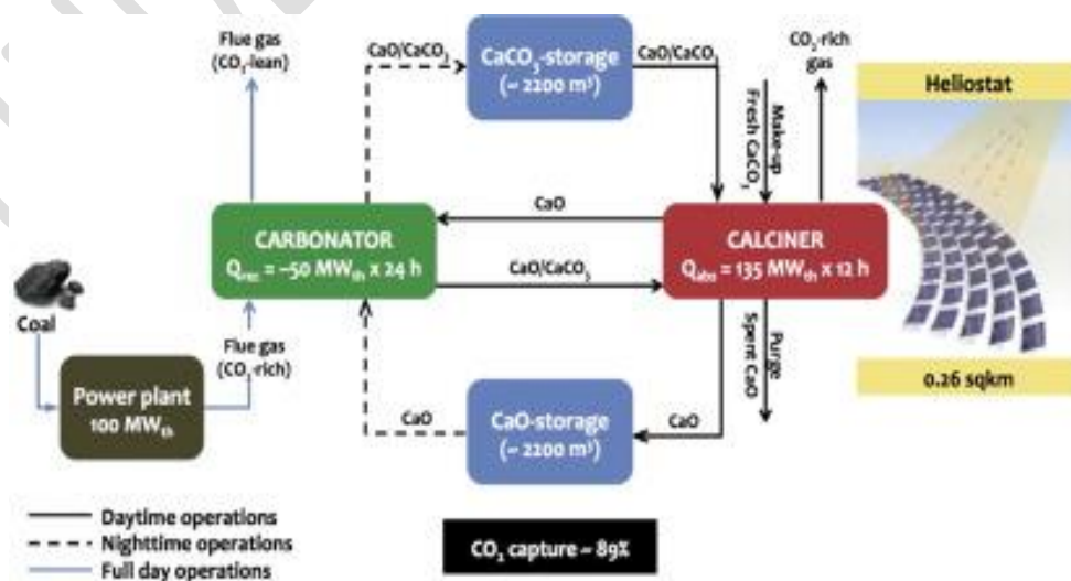
Fig 5. The calcium looping process source [46]
