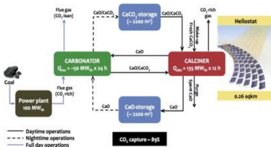
Fig 5. The calcium looping process. source [46]
