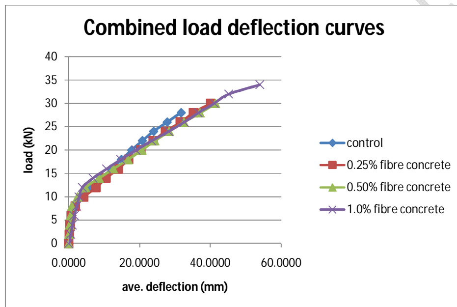
Figure 3: load deflection curves for control and fibre reinforced concretes.
