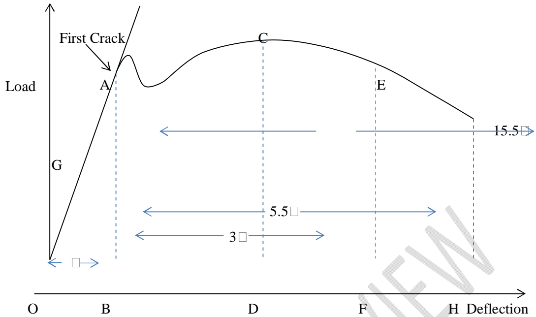
Figure 2: Analysis of Load-Deflection Curve [8]
