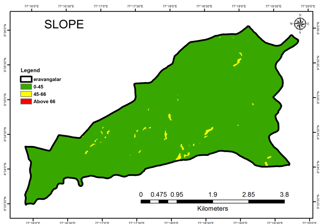
Fig. 2. Slope Map
