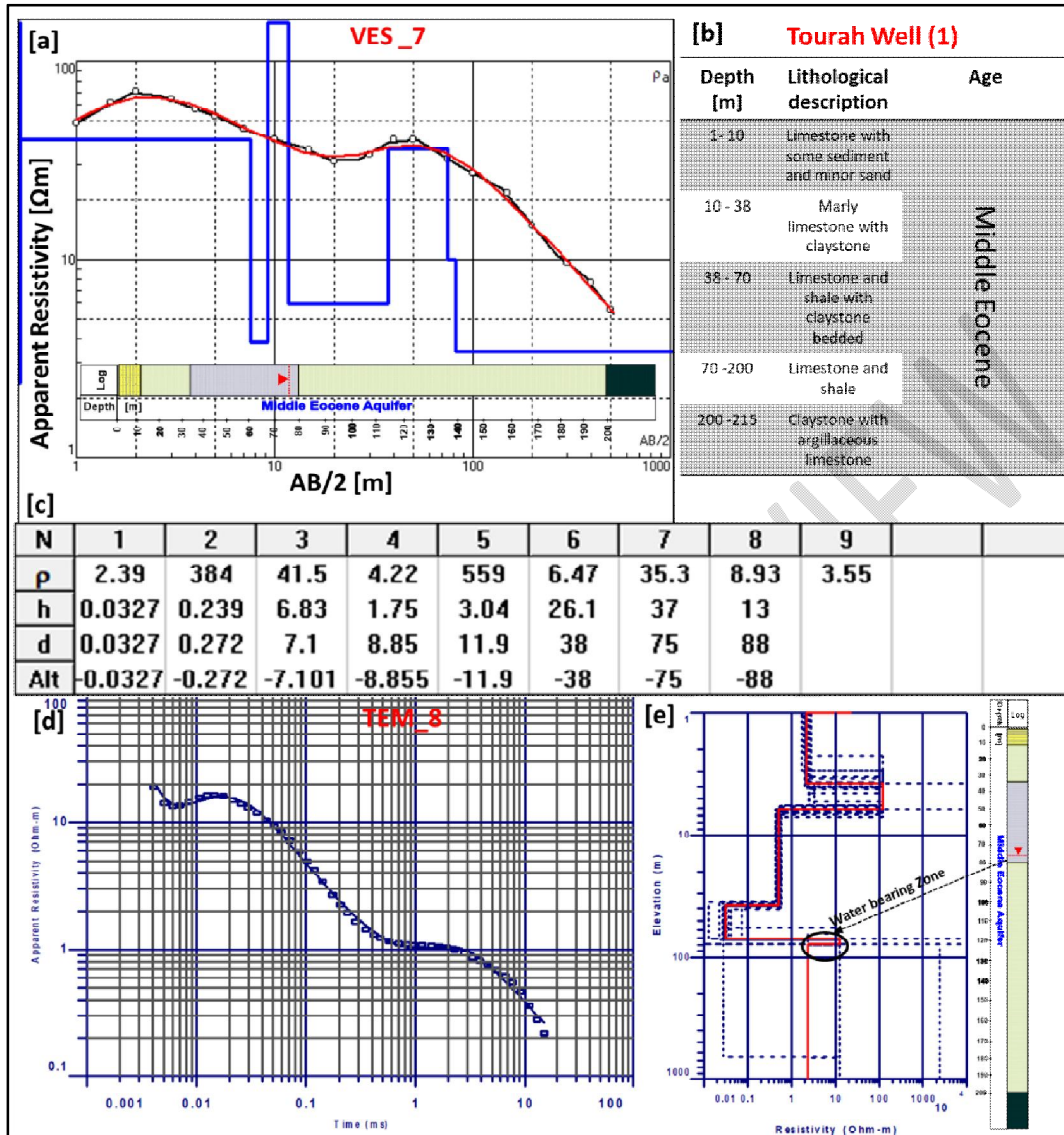
Fig. 5. Results of 1DVES and TEM soundings at the investigated site. [a] The layered model of VES no. 7 is compared with lithology of the nearby well Tourah well (1). [b] Tourah well lithology description with depth. [c] The finding of VES no.7 inversion. [d] The layered model of TEM sounding no. 8 and [e] The model layers of TEM no. 8 compared with lithology of Tourah well (1).
