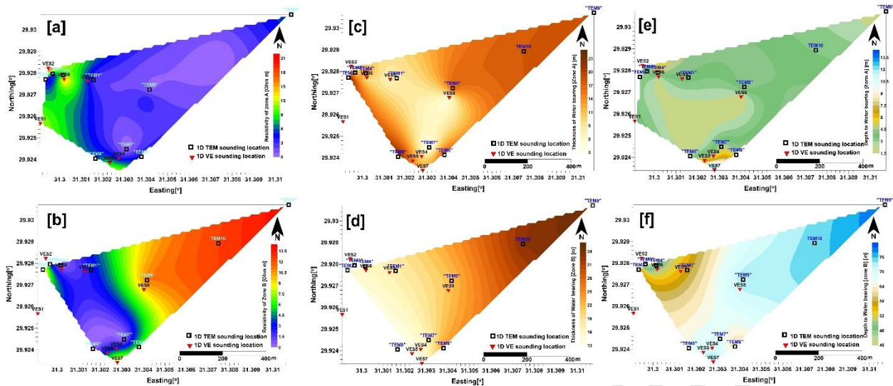
Fig .8. Iso resistivity contour maps for [a] water bearing of zones A and [b] for water bearing zone B. [c] Isopach contour maps for water bearing of zones A and [d] for water bearing zone B. [e] Depth to top of water bearing zone A where [f] Depth to water bearing zone B in the area under investigation.
