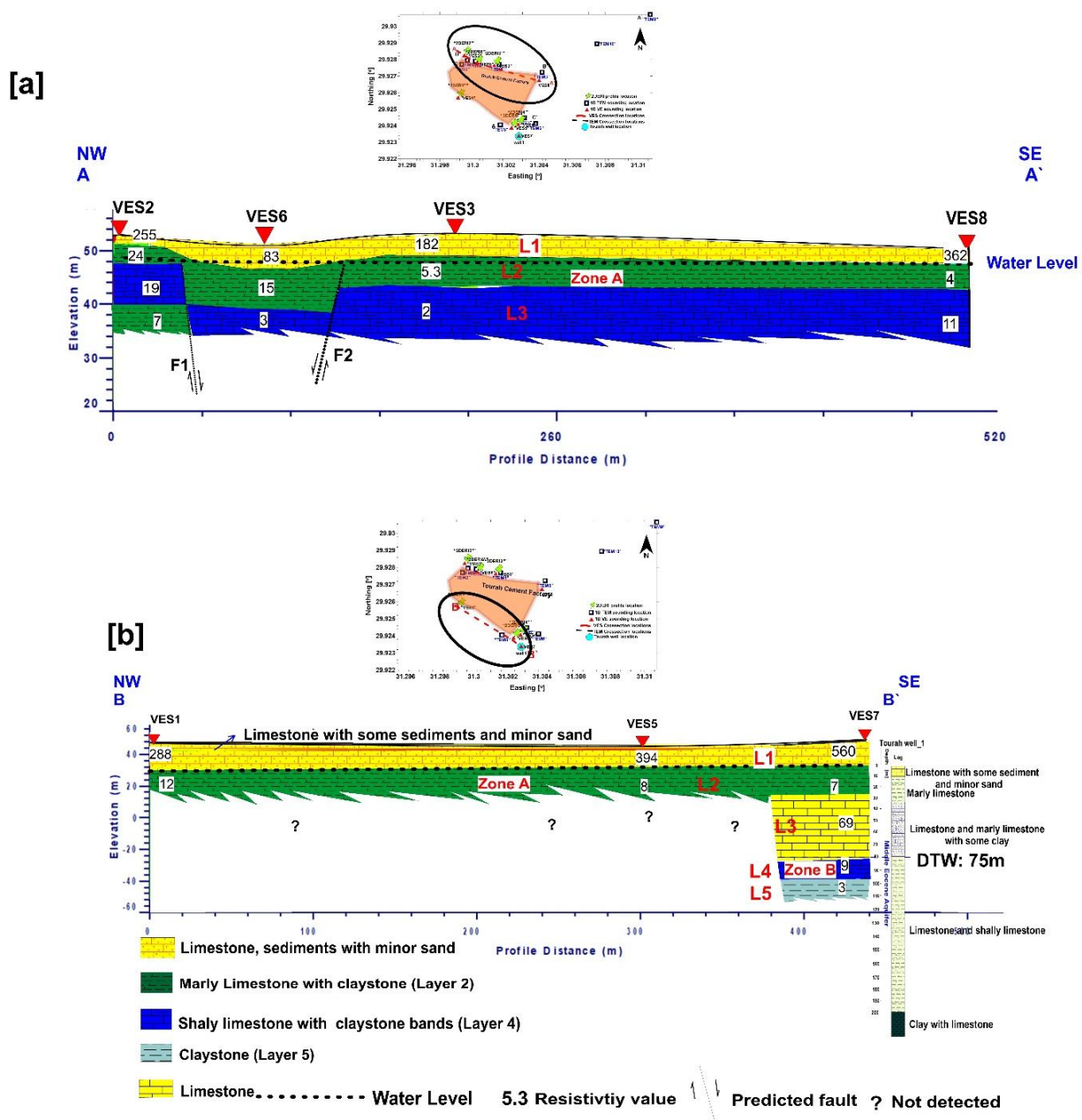
Fig. 6. Goelectrical cross sections in NW- SE direction inferred from the interpretation of 1D VES soundings measurements with the lithological of Tourah well (1). [a] Goelectrical cross section A-A`. [b] Goelectrical cross section B-B`.
