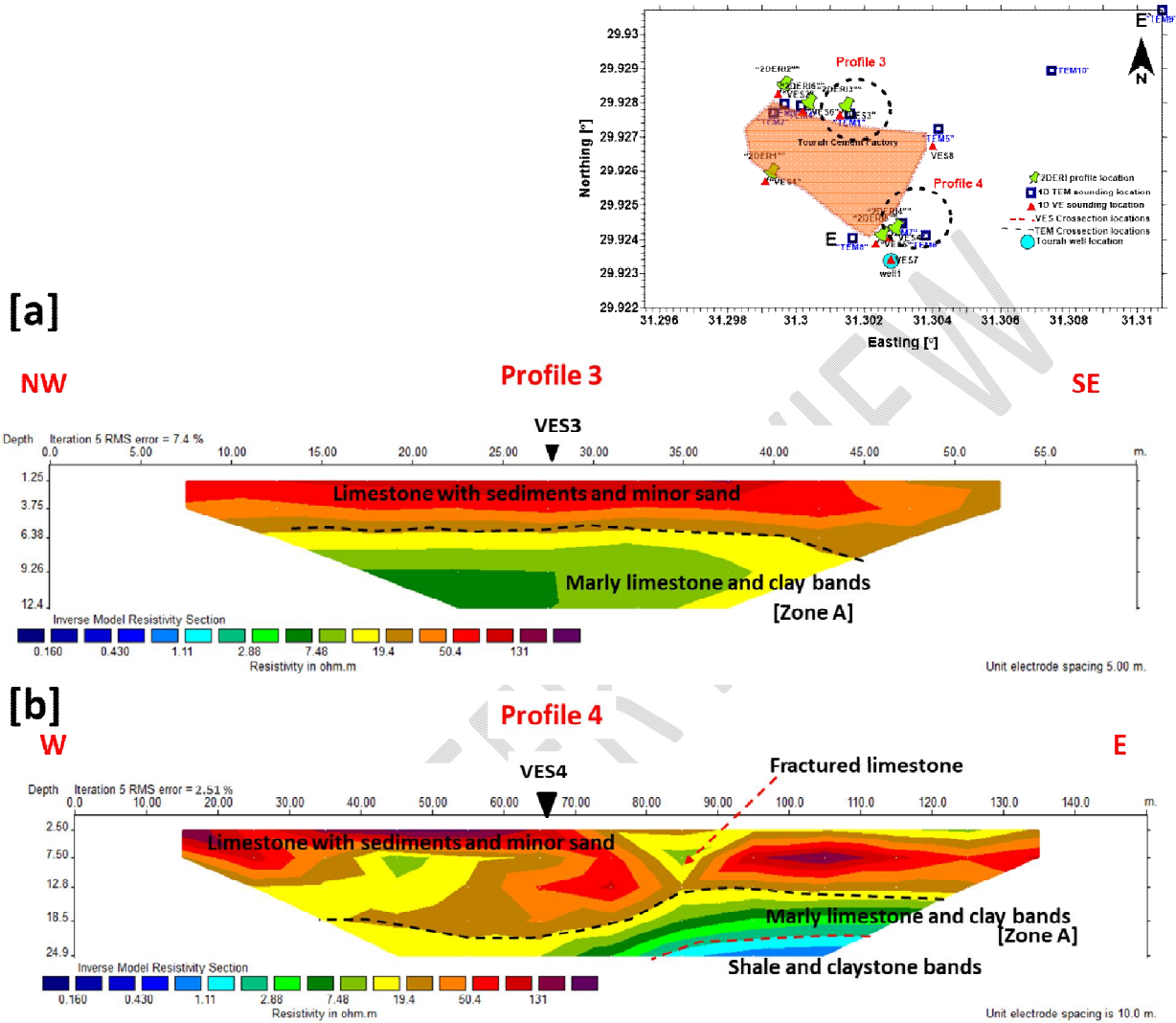
Fig. 10. 2D inversion results of 2D ERI. [a] Profile 3 in NW- SE direction[b] profile 4 in W - E direction.
