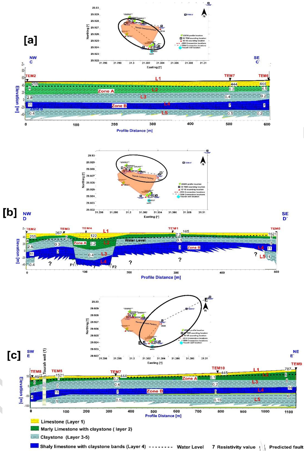
Fig. 7. Geoelectrical cross sections inferred from the interpretation of 1D TEM measurements. [a] C-C' cross section in NW-SE. [b] D-D' cross section in NW-SE and [c] E-E' cross section in SW-NE direction. L1 (layer 1), L 2 (layer 2), L 3 (layer 3), L 4 (layer 4) and L 5 (layer 5).
