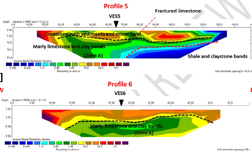
Fig. 11. 2D inversion results of 2DERI. [a] Profile 5 in NW-SE [b] profile 6 in W - E direction.
