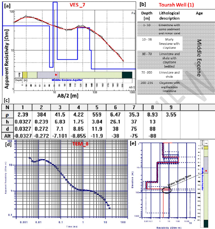
Fig. 5. Results of 1DVES and TEM sounding at investigated site. [a] The layered model of VES no.7 is compared with lithology of the nearby well Tourah well (1). [b] Tourah well lithology description with depth. [c] The finding of VES inversion. [d] The layered model of TEM sounding no.8 and [e] The model layers of TEM no.8 compared with lithology of Tourah well (1).
