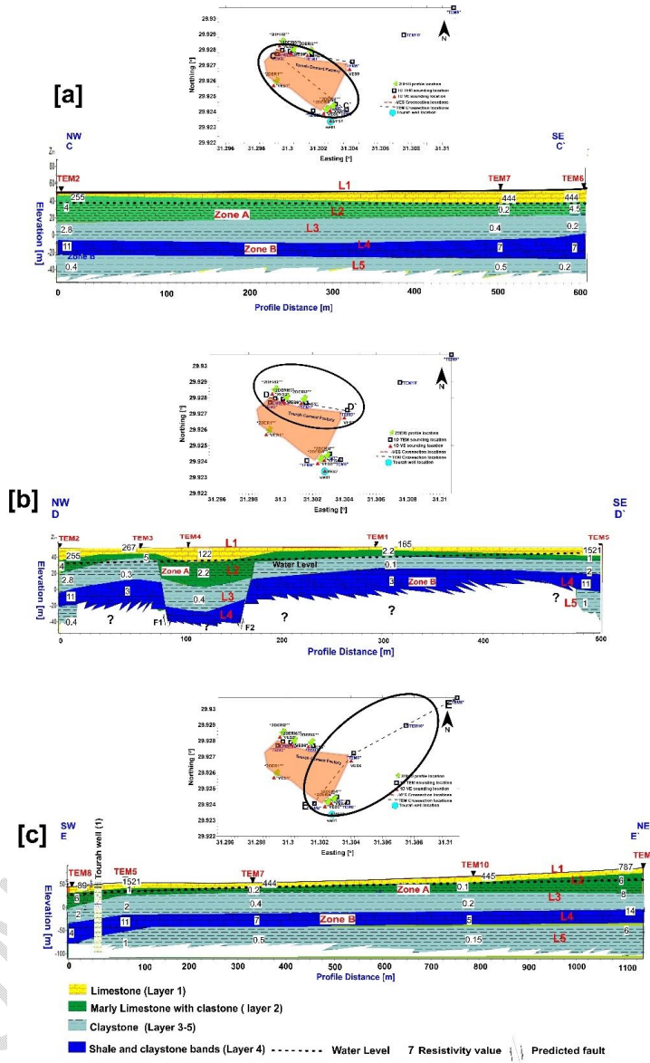
Fig. 7. Geoelectrical cross sections inferred from the interpretation of TEM measurements. [a] C-C' cross section in NW-SE. [b] represent D-D' cross section in NW-SE and [c] E-E' cross section in SW-NE direction. L1(layer 1), L 2 (layer 2), L 3 (layer 3), L 4 (layer 4) and L 5 (layer 5).
