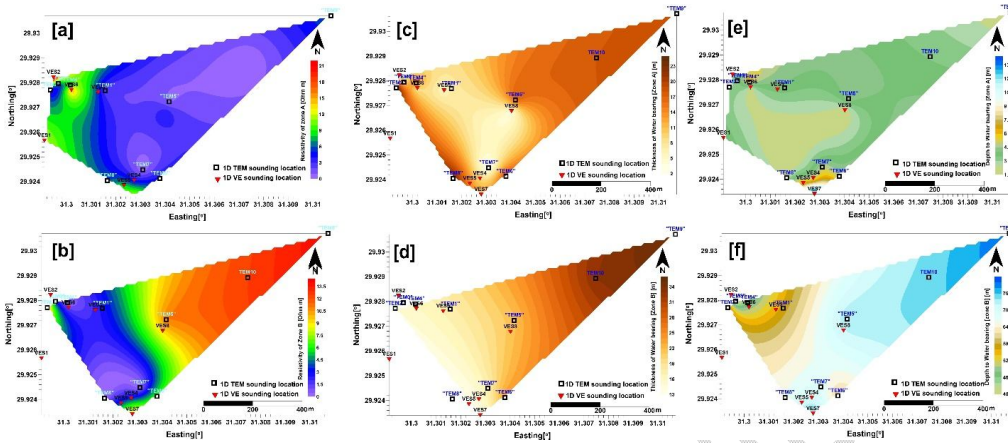
Fig. 8. Iso resistivity contour maps for [a] waterbearing of zones A and [b] for waterbearing zone B. [c] Isopach contour maps for waterbearing of zones A and [d] for waterbearing zone B. [e] Depth to top of waterbearing zone A where [f] Depth to of waterbearing zone B in the area under investigation.
