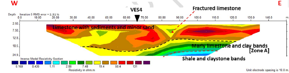
Fig. 10. 2D inversion results of 2DERI [a] Profile 3 in NW- SE direction[b] profile 4 in W - E direction.
