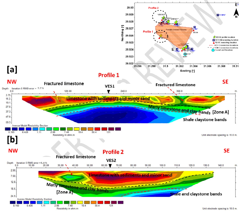
Fig. 9. 2D inversion results of 2DERI. [a] Profile 1. [b] profile 2 in NW-SE direction.
