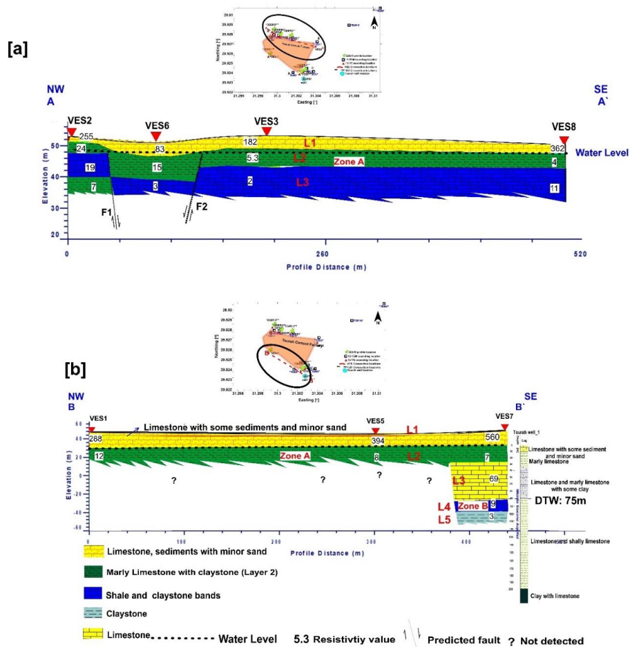
Fig. 6. Geoelectrical cross sections in NW- SE direction inferred from the interpretation of VES soundings measurements with the lithological of Tourah well (1). [a] Geoelectrical cross section A-A'. [b] Geoelectrical cross section B-B'.
