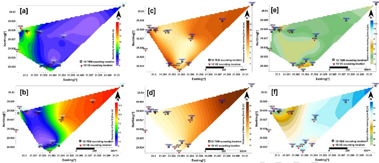
Fig. 8. Iso resistivity contour maps for [a] waterbearing of zones A and [b] for waterbearing zone B. [c] Isopach contour maps for waterbearing of zones A and [d] for waterbearing zone B. [e] Depth to top of waterbearing zone A where [f] Depth to of waterbearing zone B in the area under investigation.
