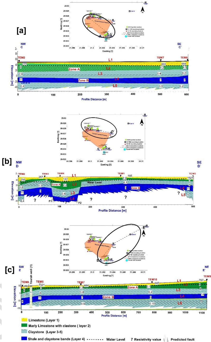
Fig. 7. Geoelectrical cross sections inferred from the interpretation of TEM measurements. [a] C -C` cross section in NW-SE. [b] represent D-D` cross section in NW-SE and [c] E-E` cross section in SW-NE direction. L1(layer 1), L 2 (layer 2), L 3 (layer 3), L 4 (layer 4) and L 5 (layer 5).
