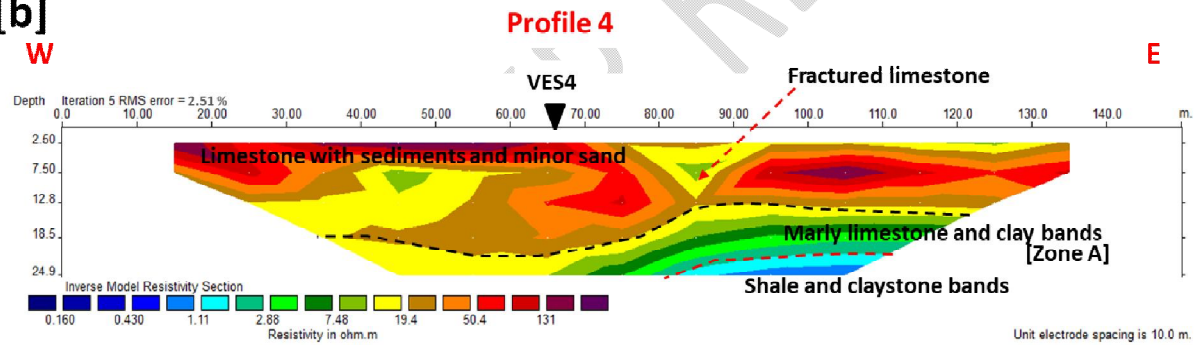
Fig. 10. 2D inversion results of 2DERI. [a] Profile 3 in NW- SE direction[b] profile 4 in W - E direction.
