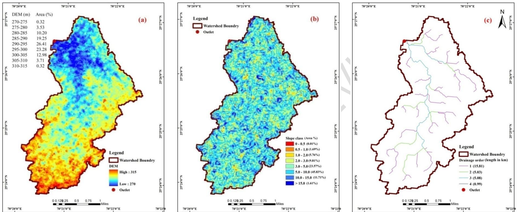
Fig. 2. Digital Elevation Model (a), slope (b) and drainage (c) maps of Parasai-Sindh watershed
