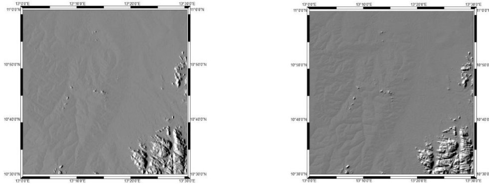
Fig 2a-h). Hill shaded image of azimuths 0°, 45°, 90°, 135°, 180°, 225°, 270°, and 315° respectively.
