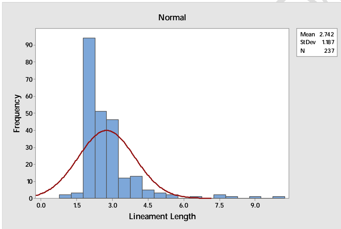
Fig. 5: Histogram of the total lineament of the study area.
