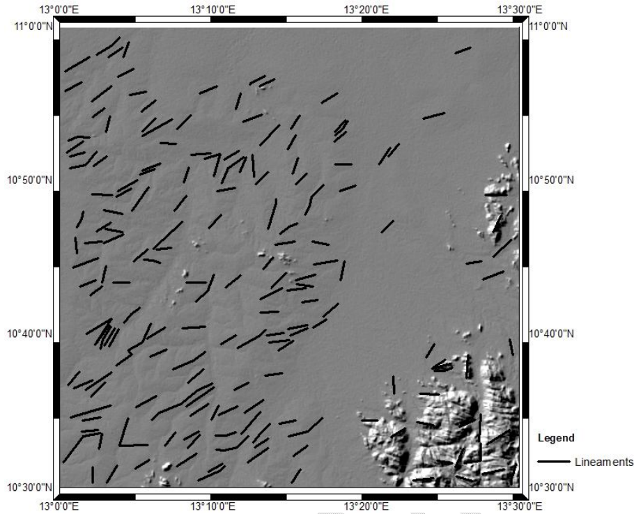
Fig. 3b) Combined hill-shade image of azimuth 180^\circ , 225^\circ , 270^\circ , and 315^\circ with the automatically extracted lineaments
