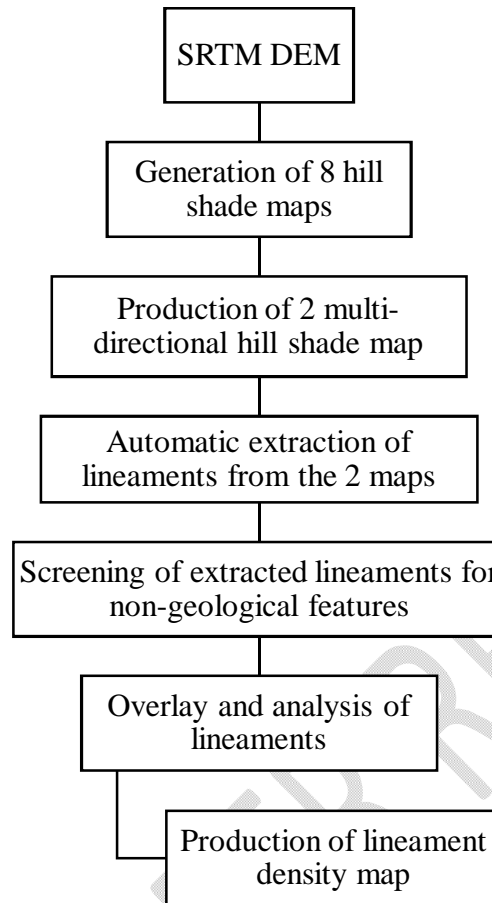
Fig. 1: Flowchart of lineaments extraction
