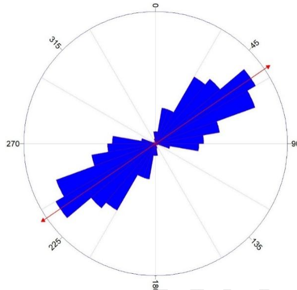
Fig. 6: Rose diagram of the lineament map
