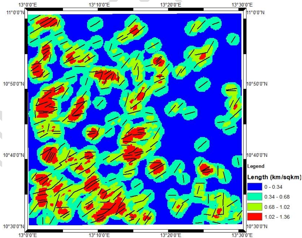
Fig. 7: Lineament density map of the study area
