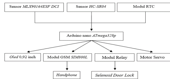
Figure 3. Block diagram of measuring instrument design.
