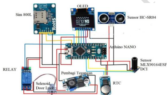
Figure 2. Design of a series of tools.
