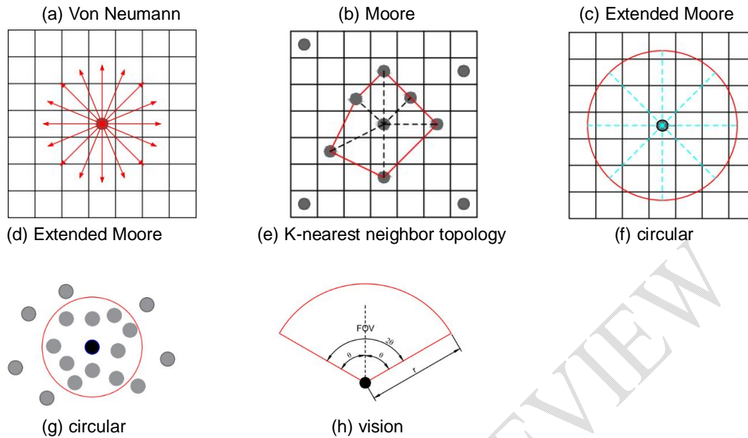
Fig.1(A-H).Range of pedestrian interaction in different models
