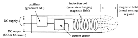
Figure 3 Drawing of Poximity Inductive Sensor Circuit.
