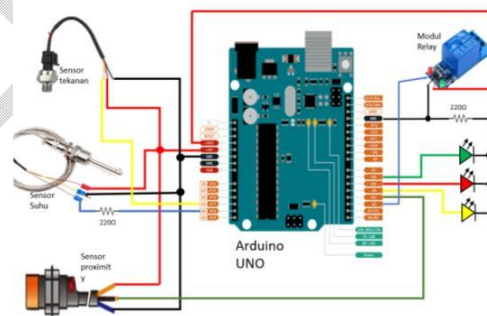
Figure 5 Arduino Circuit
