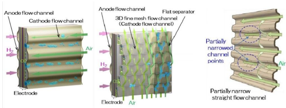
Figure 5 shows the Toyota Mirai's flow field architecture[25]
