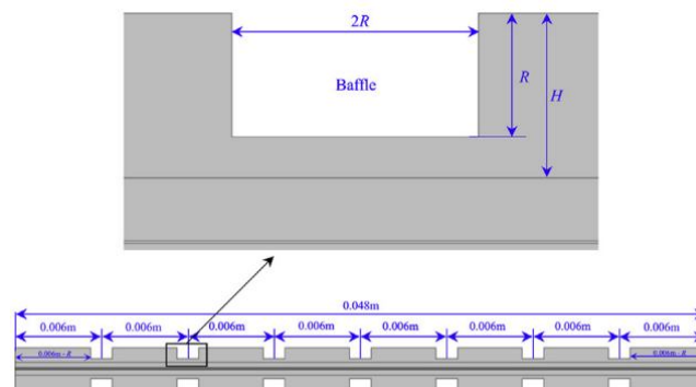
Figure 4 Model of the two-dimensional PEMFC by Chen[22]
