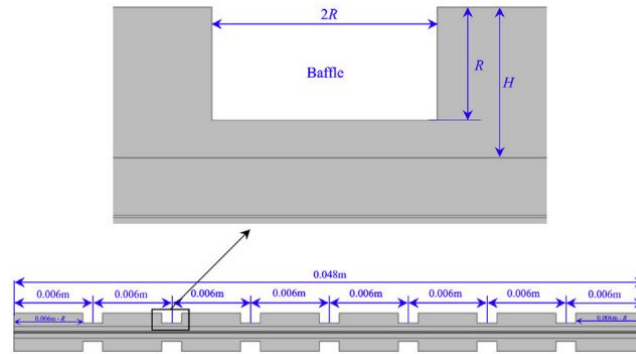
Figure 3 Model of the two-dimensional PEMFC by Chen (ref required)
