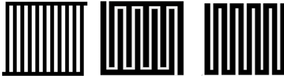
Figure 2 (a) Parallel flow field (b) Alternating finger flow field (c) Serpentine flow field
