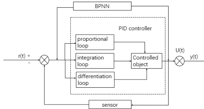
Figure 2 BP neural network PID controller structure
