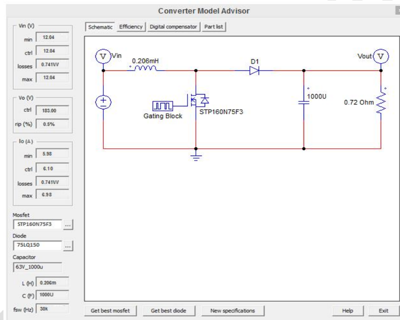
Fig. 2. Implementation of the DC-DC converter model
