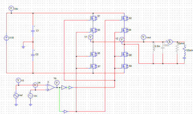
Fig. 4. Simulated inverter system
