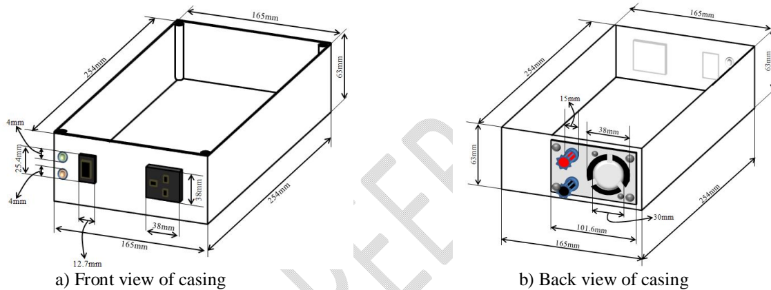
Fig. 10. Isometric representation of the casing (front and back view)
