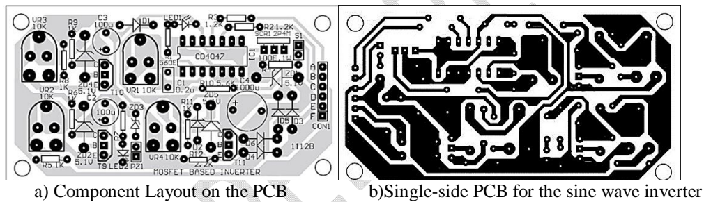
Fig. 8. Component layout on the PCB and single-side PCB for the sine wave inverter circuit
