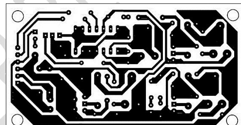
b) Single-side PCB for the sine wave inverter
