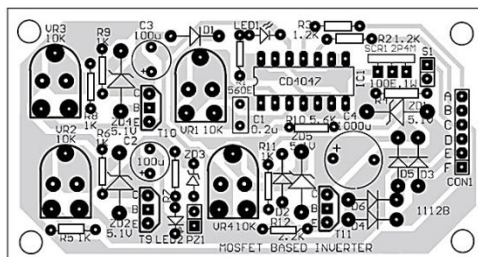
a) Component Layout on the PCB
