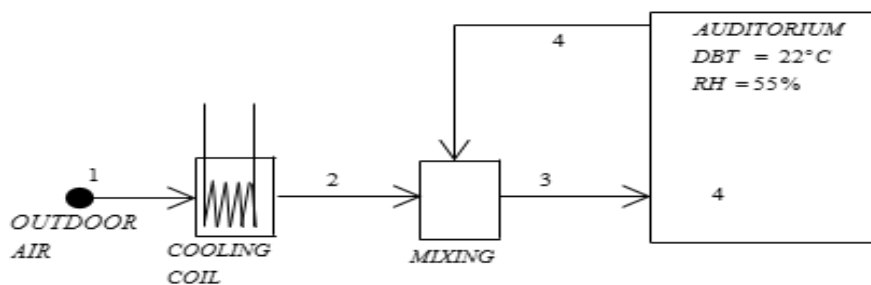
Figure 1(a): Block diagram representation of the auditorium air-conditioning problem.
