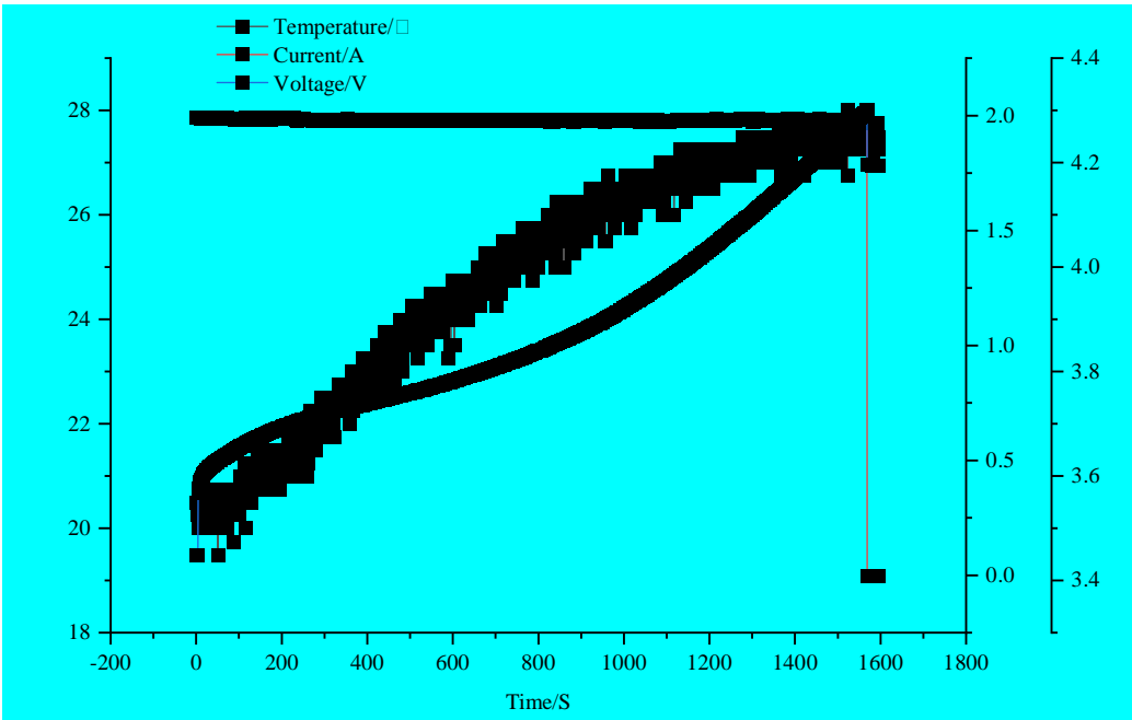
Figure 5 Battery parameter change
