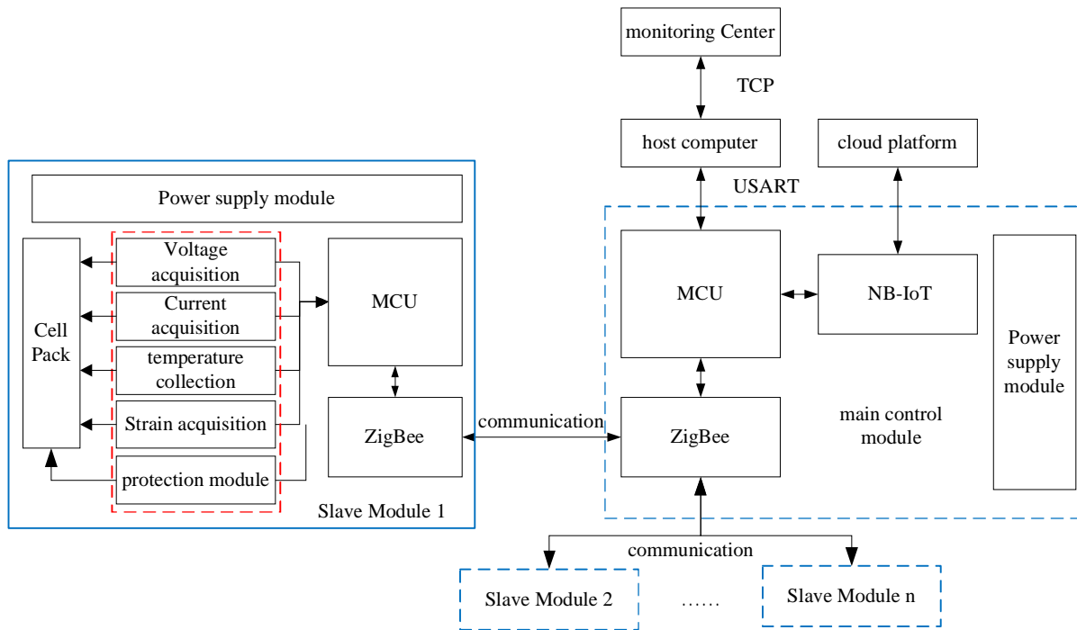
Fig.2.Hardware structure diagram
