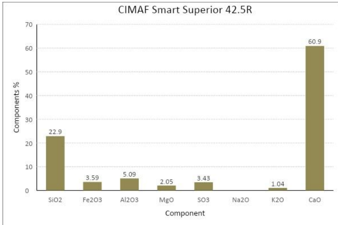
Fig. 6. Chemical composition of CIMAF Smart Superior 42.5R
