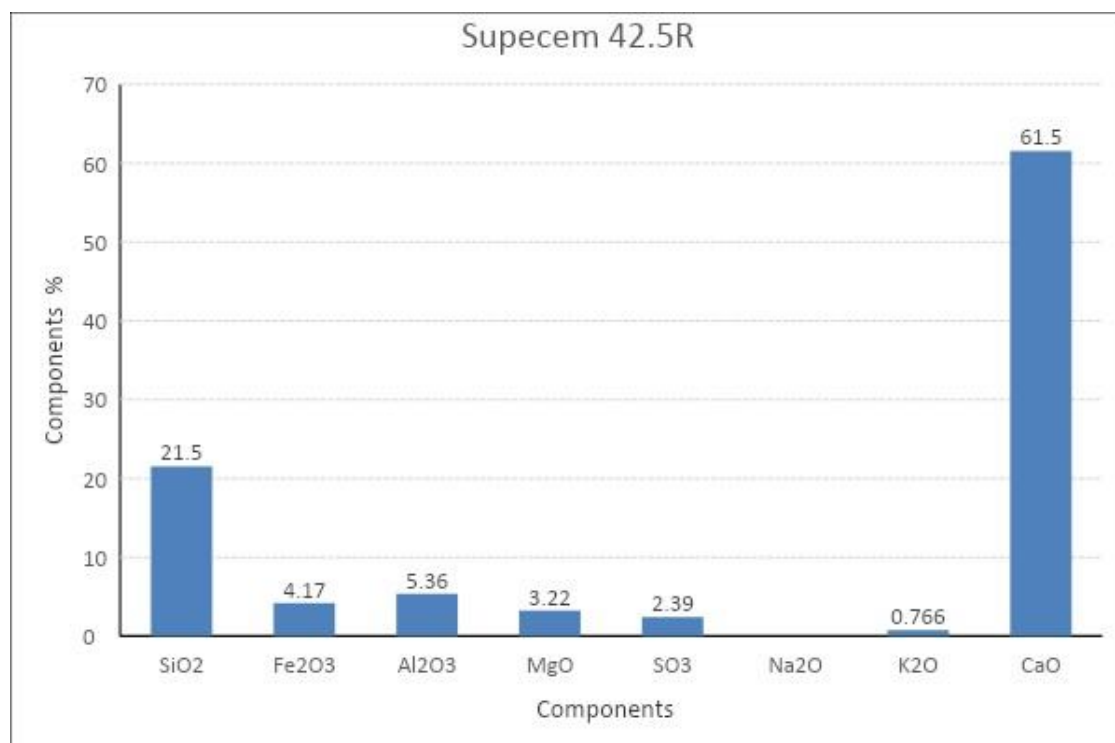
Fig. 11. Chemical composition of Supacem 42.5R
