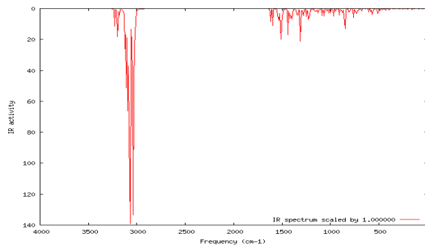
(b) Bromine doped P3HT
