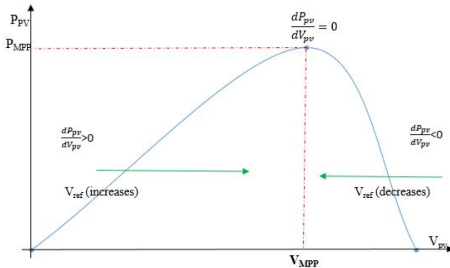
Figure 5: P-V Characteristics of PV panel [6]
