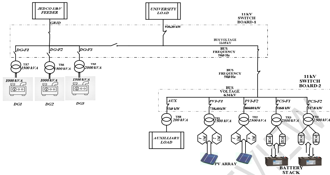
Figure 1: Single Line Diagram of JOSTUM 3.5 MW SHPP
