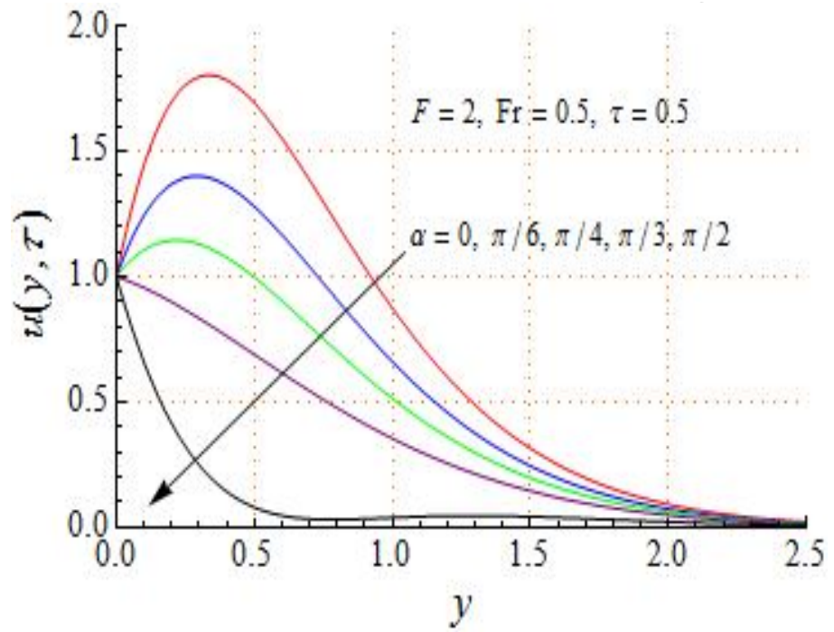
Figure 4. Velocity profile on varying \alpha
