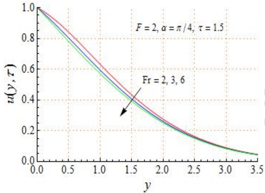
Figure 2. Velocity profile on varying Fr (large)
