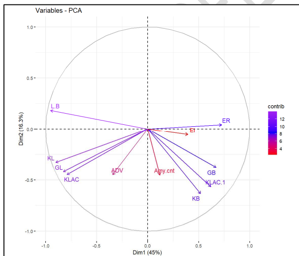
Figure 2. Principle component analysis biplot traits
