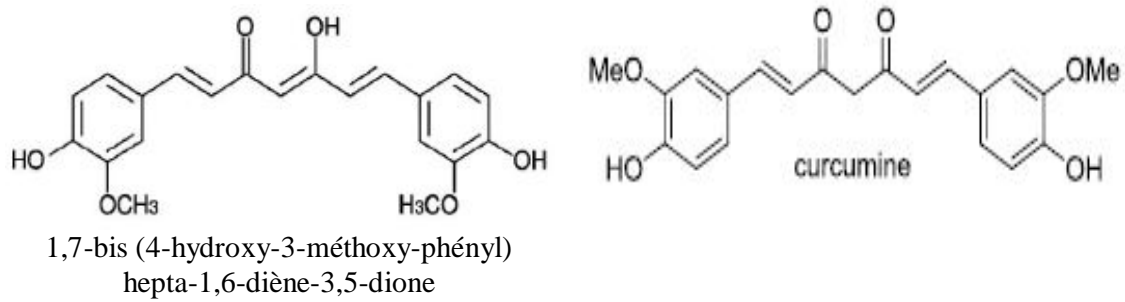
Fig. 1 : Chemical structure of curcumin :
