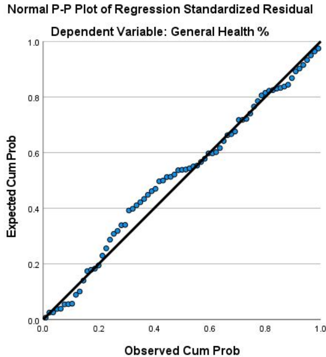
Figure 2: Normal-PP plot for regression residual
