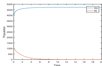
Figure 1: \eta = 2.5 , \epsilon = 0.25
