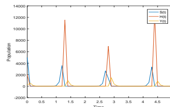
Figure 4: p_1 = 0.4, \mu = -0.14, \epsilon = 0.001
