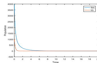
Figure 2: \eta > 3 , \epsilon = 5
