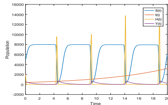
Figure 6: r = 4.8, d = 1, \eta = 1.3
