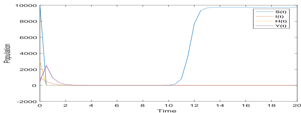
Figure 8: In the absence of Allee effect
