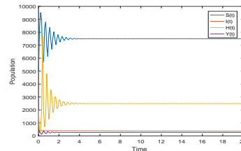
Figure 7: \eta = 0.2, d = 6
