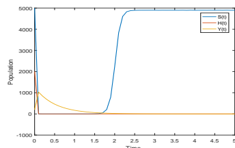
Figure 3: p_1 = 4, \mu = 0.2, \epsilon = 0.1
