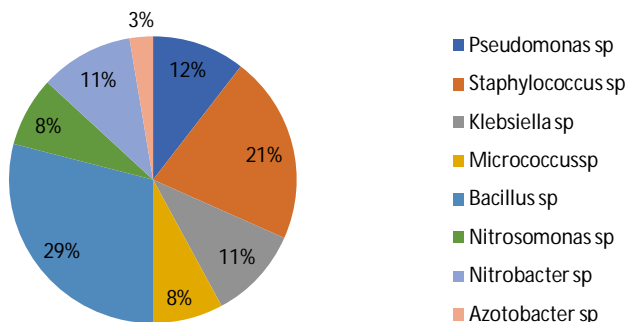
Fig 4: Percentage Occurrence
