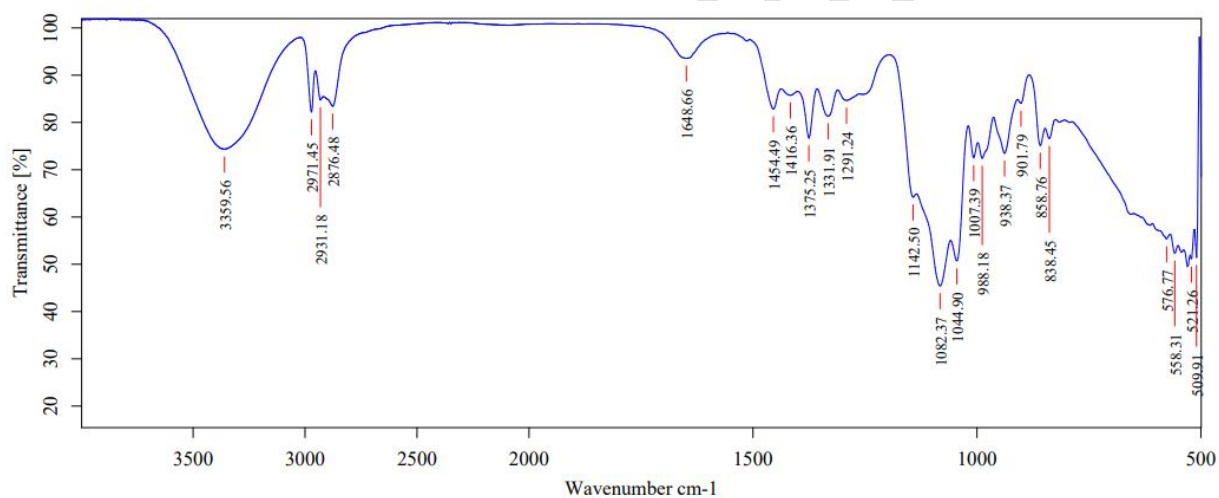
FIGURE-3 FTIR spectra of Clove oil
