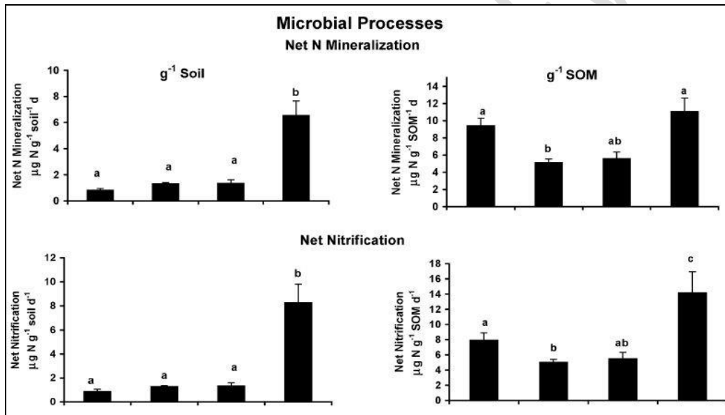
Fig 2: Microbial processes including net mineralization g^{-1} soil and g^{-1} SOM (error bars represent standard error). Different letters above bars represent statistically significant differences at P=0.05 .
