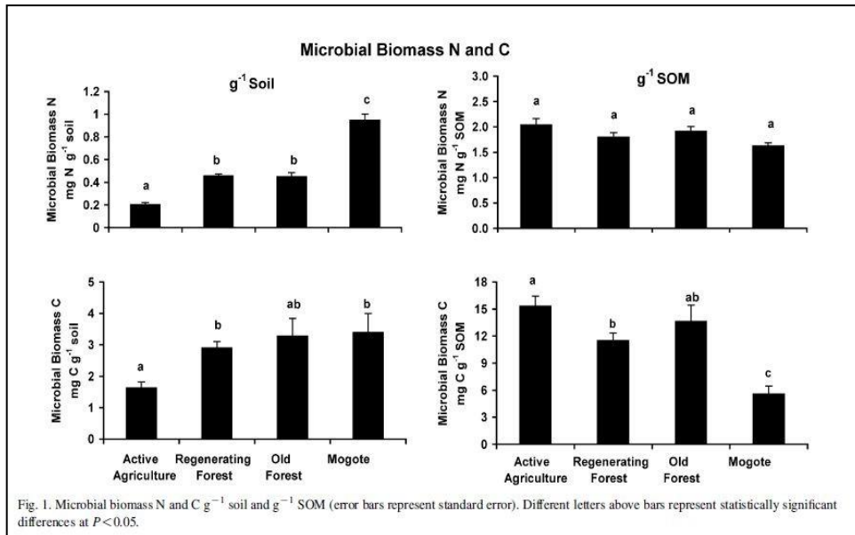
Fig 1: Microbial biomass N and C g -1 soil and g -1 SOM (error bars represent standard error). Different letters above bars represent statistically significant differences at P = <0.05.
