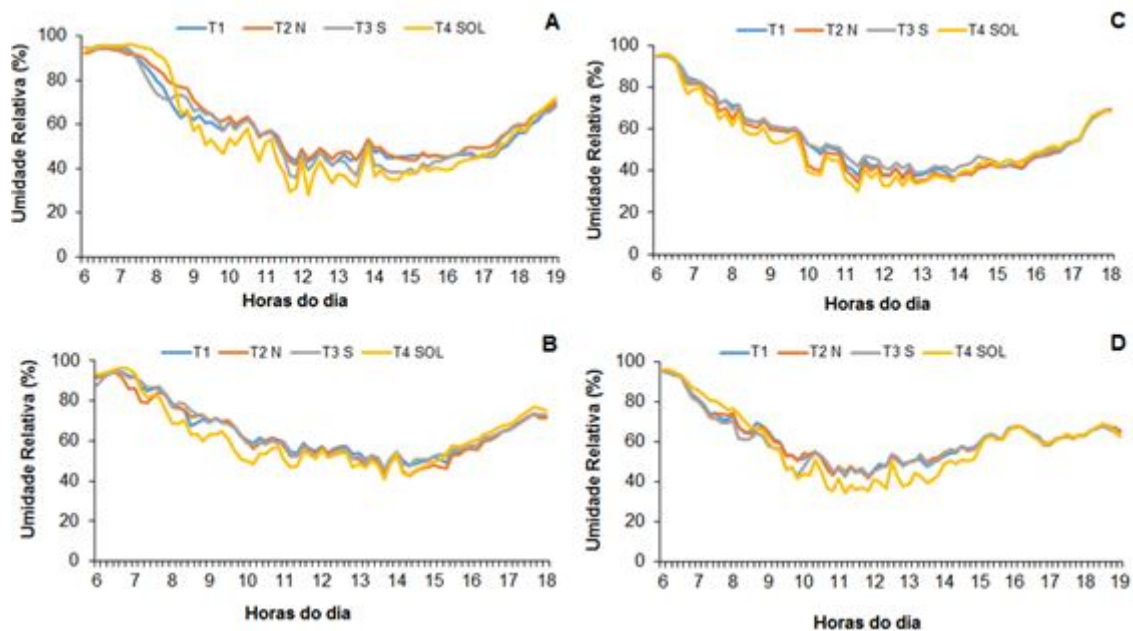
Fig. 13. Daily values of Relative Humidity in Summer (A), Autumn (B), Winter (C) and Spring (D), in Papaya planted in the East-West direction, where: T1: located in the papaya planting line; T2 N: located 40 cm from the planting line on the north side; T3 S: located 40 cm from the planting line on the south side; T4 Sun: located in the full sun planting row.
