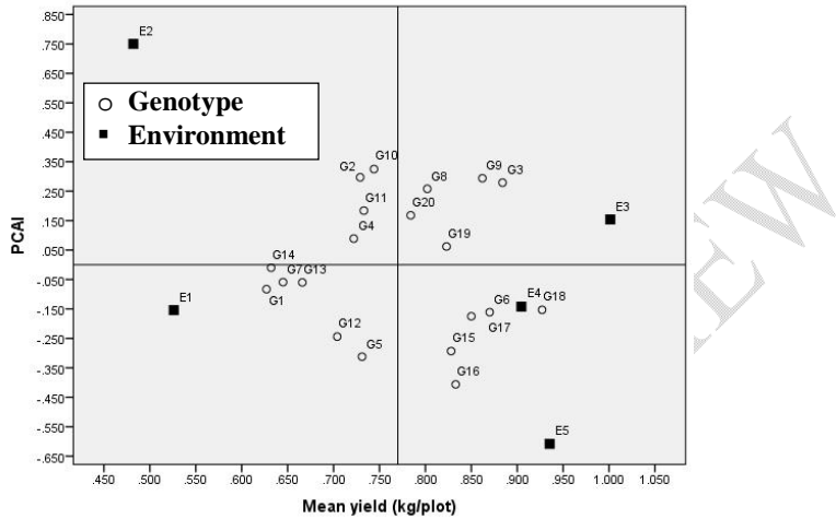
Figure 1 : AMMI1 biplot for black gram genotypes and locations.
