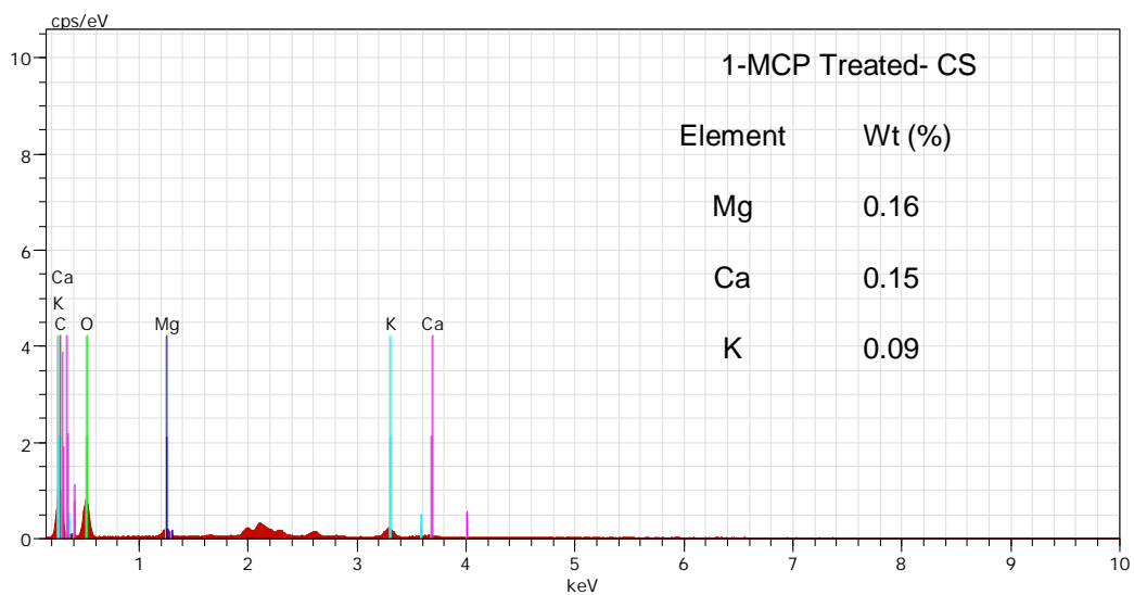
Fig. 5b EDAX analysis of Mg, Ca and K (%) 1-MCP treated and control sample under CS
