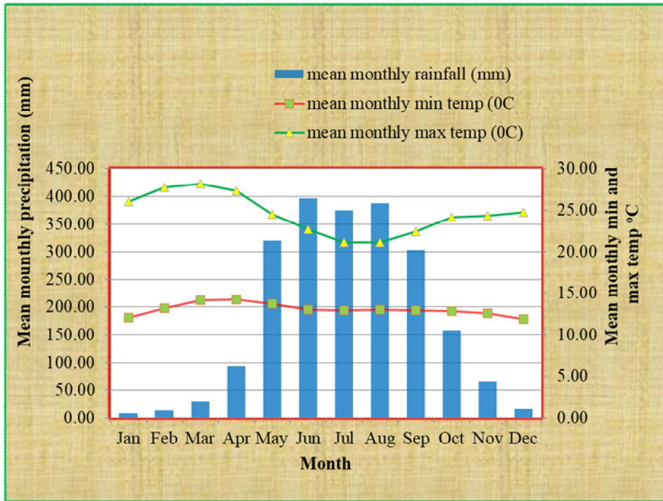
Figure 12: Mean monthly rainfall, maximum and minimum temperatures of the study area for the years 2006 – 2018. (Nekemte Meteorological Station).
