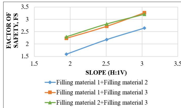
231 232 Fig. 9. Slope Vs Safety Factor for Embankment considering two filling materials (H= 12 m) 233
