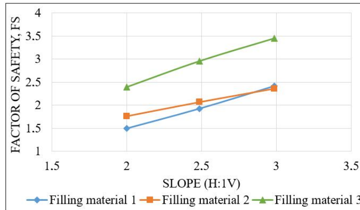
Fig. 7. Slope Vs Safety Factor Embankment has different Filling materials and 17 m Height
