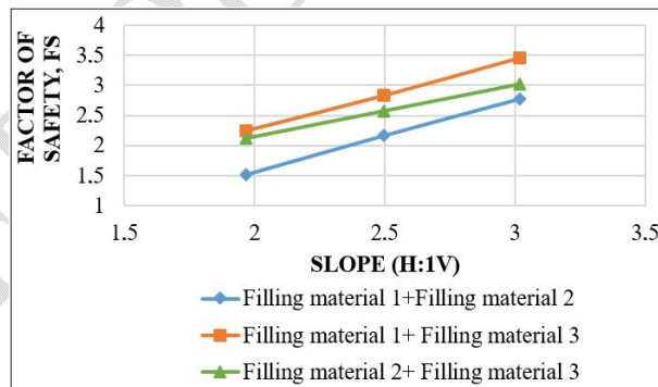
237 238 Fig. 10. Slope Vs Safety Factor for Embankment considering two soil layers once H= 17 m 239
