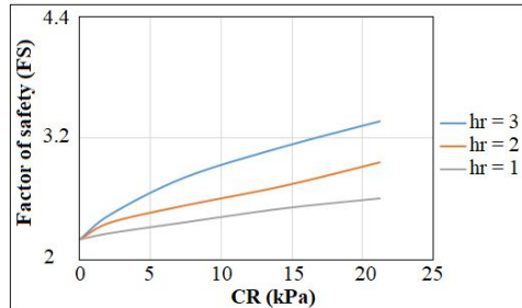
Fig. 12. Factor of safety variation when vetiver vegetation Spreading on the Whole ground surface ( c' = 5 ).
