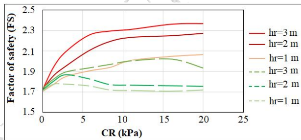
Fig. 11. Factor of safety variation with confined vegetation in the slope surface only ( c' = 5 ).
