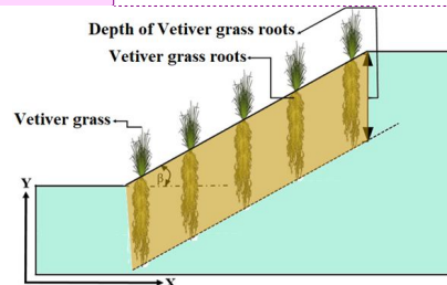
Fig. 3. Root Reinforcement Model
