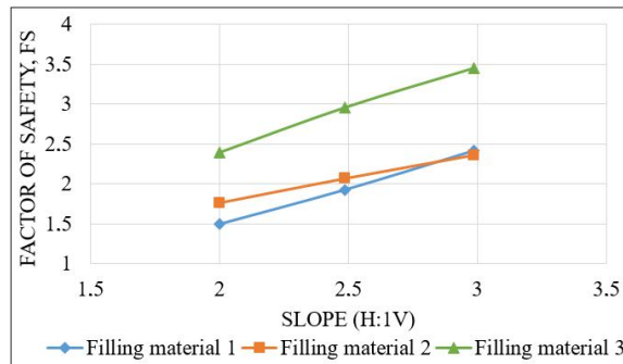
Fig. 7. Slope Vs Safety Factor Once Embankment has different Filling materials and 17 m Height. All the safety factor values observed in Table 4 and Figure 7 are superior to 1.5 regardless the soil type and homogeneous embankment slope. The lowest value remains 1.51. The difference among safety factors remains the same which previously perceived above. Less distance can be noticed among curves.
