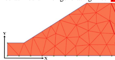
Fig. 2. Mesh generation
