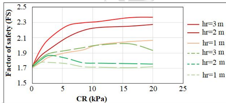
Fig. 11. Factor of safety variation with confined vegetation in the slope surface only ( c' = 5 ).
