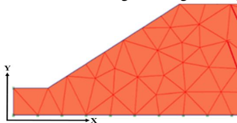
Fig. 2. Mesh generation
