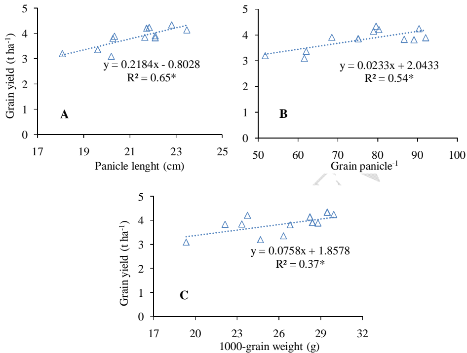
Fig. 3. Relationship of grain yield of rice with yield panicle length (A), Grain panicle -1 (B) and 1000-grain weight (C)
