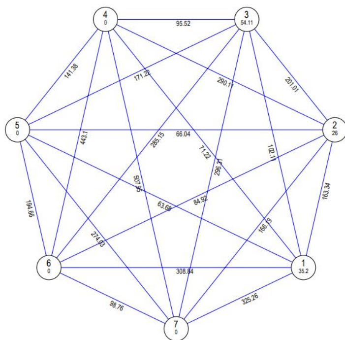
Mahalanobis Euclidean Distance (Not to the Scale)
