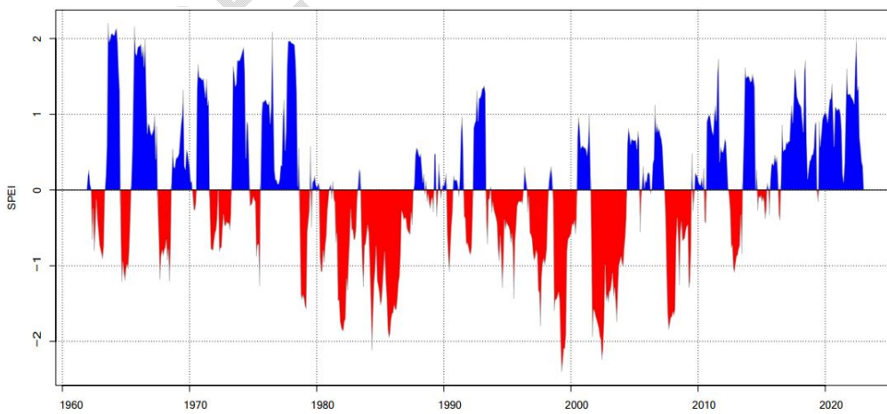
c) SPEI at 12 months accumulation time scales for Massili Basin
