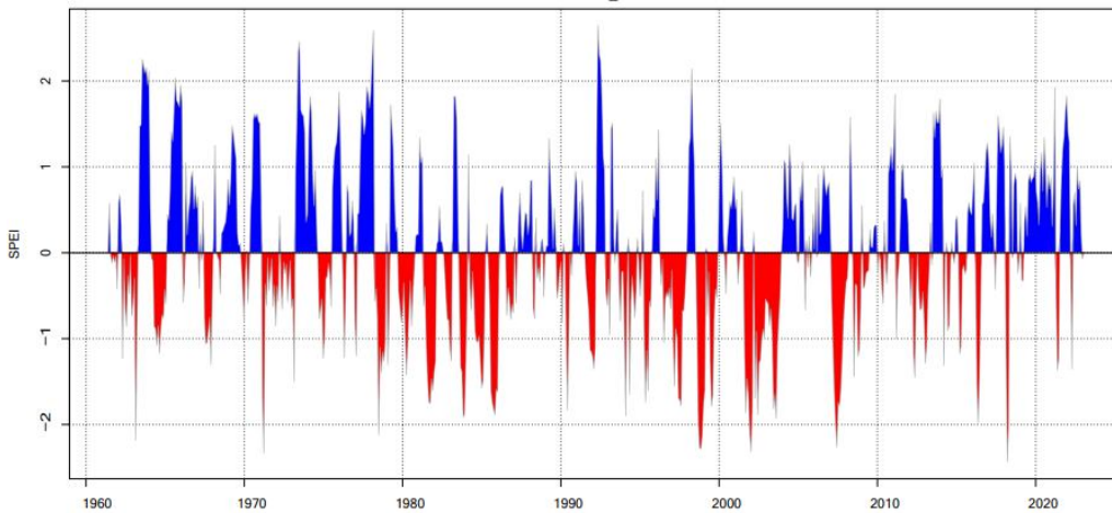
b) SPEI at 6 months accumulation time scales for Massili Basin
