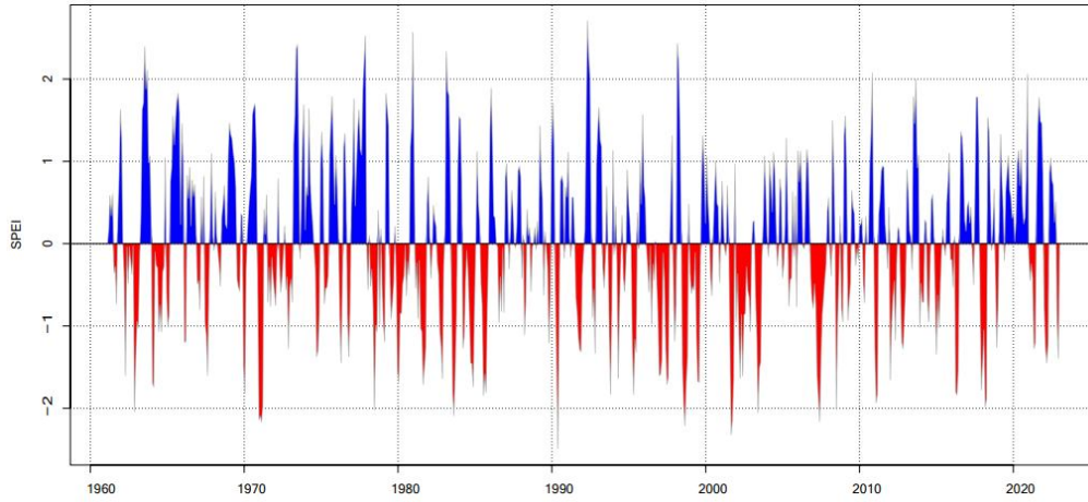
a) SPEI at 3 months accumulation time scales for Massili Basin
