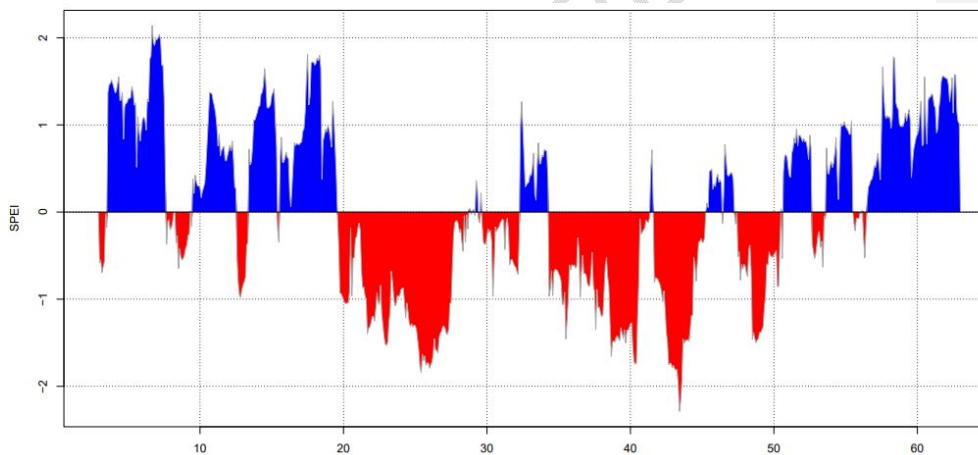
d) SPEI at 24 months accumulation time scales for Massili basin
