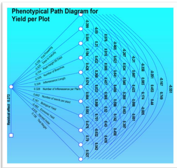
Fig: 03. Phenotypic Path Diagram for yield plot -1
