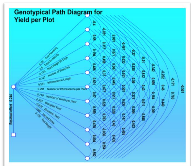
Fig: 04. Genotypic Path Diagram for yield plot -1
