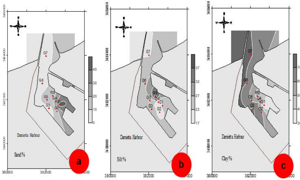
Fig. 4. Geographical distribution of a) sand%, b) silt% and c) clay% of Grab samples in the Damietta harbor basin
