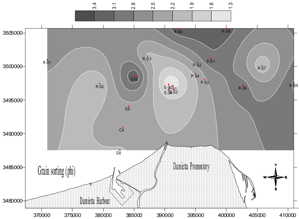
Fig 10. Offshore geographical distribution of grain sorting (standard deviation) in phi unit
