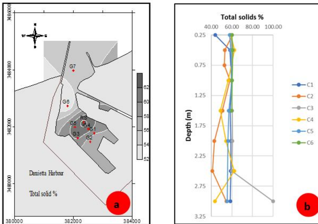
Fig. 11. Geographical distribution of total solids % (a. the Grab samples in the Damietta harbor basin, and b. Total solids % distribution of the Core samples)
