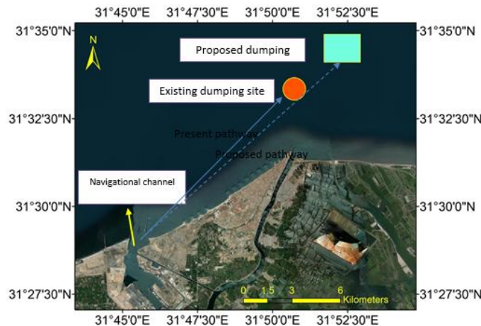
Fig. 20. Offshore existing and proposed offshore dumping sites
