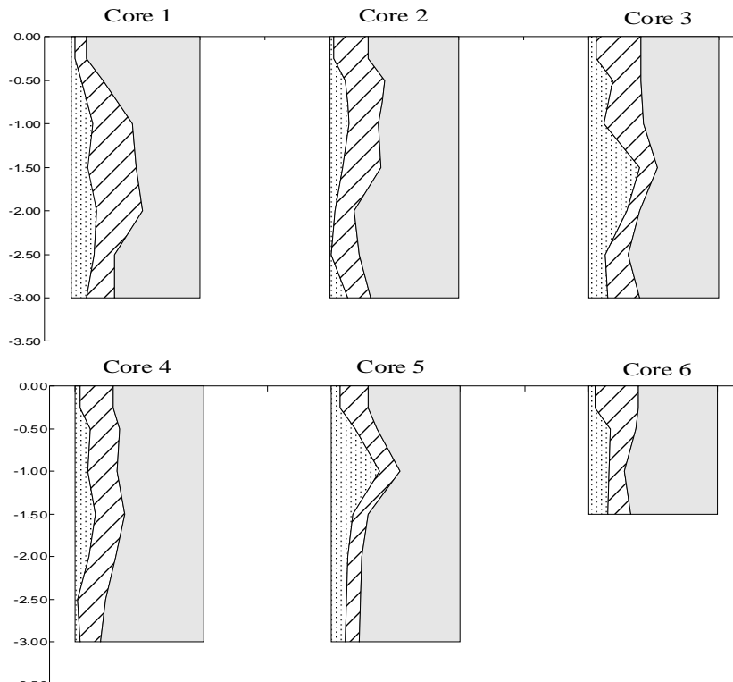
Fig. 5. Vertical distribution of sand %, silt%, and clay% in the examined cores
