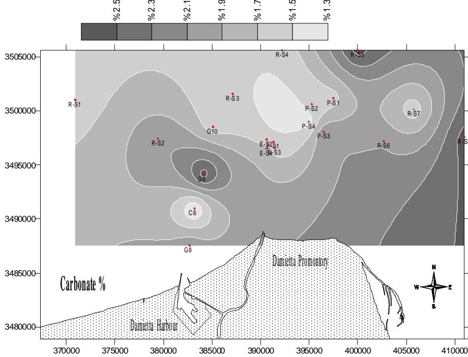
Fig. 14. Offshore geographical distribution of carbonate %
