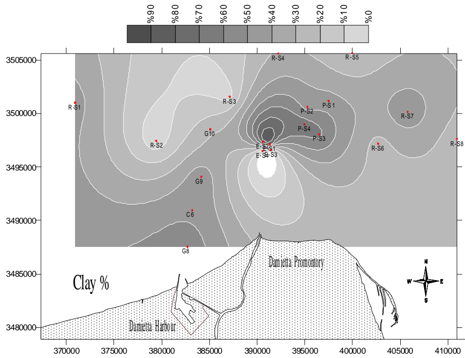
Fig. 8. Offshore geographical distribution of a) sand%, b) silt% and c) clay% of Damietta
