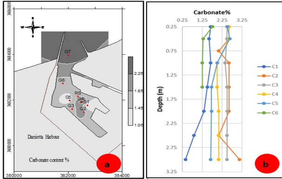
Fig. 13. Geographical distribution of carbonate content % (a. Grab samples in the Damietta harbor basin and b. Carbonate content % distribution of the core samples)
