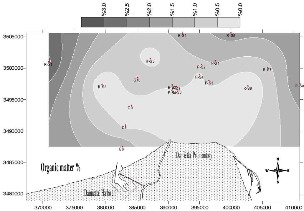
Fig. 16. Offshore geographical distribution of organic matter %
