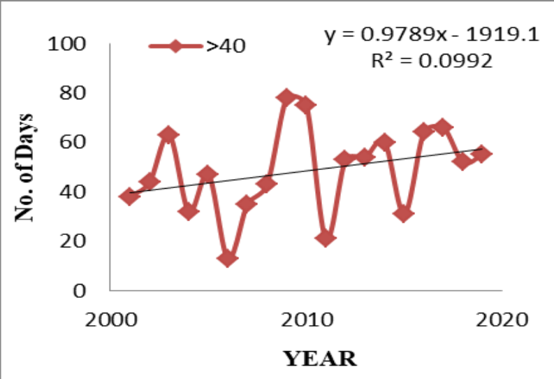
Fig.3 Trend of extreme temperature in Sambalpur district
