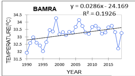
Fig.2 Trend of maximum temperature in all the blocks of Sambalpur district
