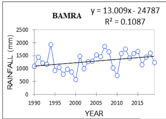
Fig.1 Trend of seasonal rainfall in all the blocks of Sambalpur district
