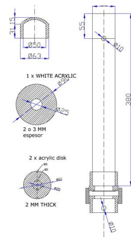
Figure 8 design of GOES plankton sampler
