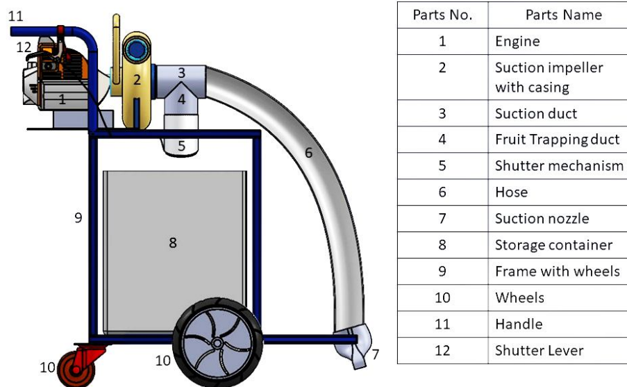
Fig. 4. Conceptual drawing of the machine prototype.
