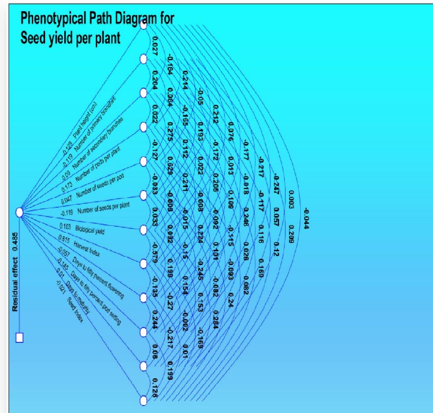
Fig 2: PHENOTYPIC PATH DIAGRAM
